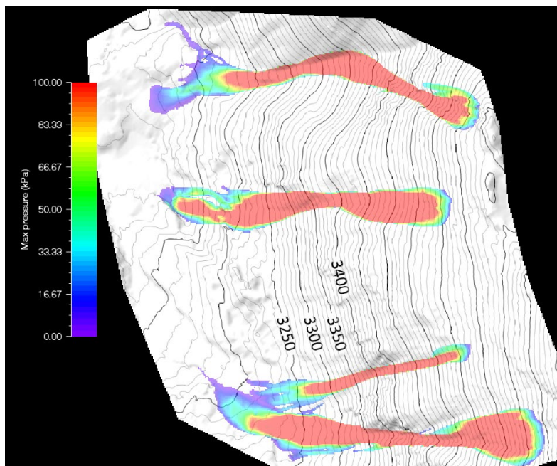
Run 43 – pressure
