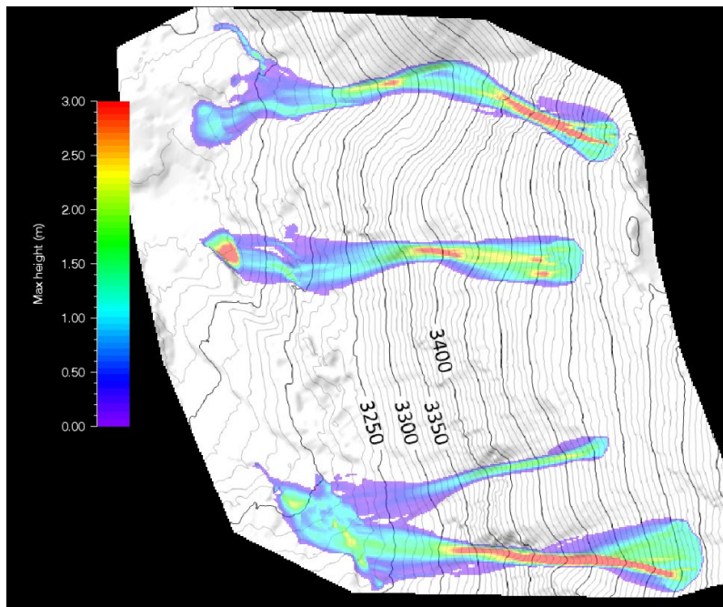
Run 43 – height
