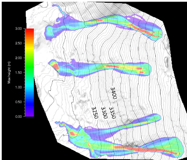
Run 44 – height
