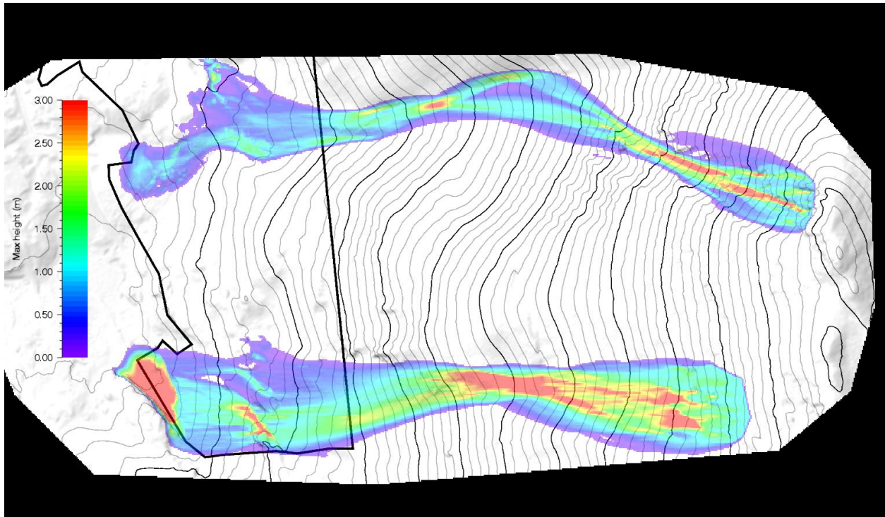
Run 36 – height
