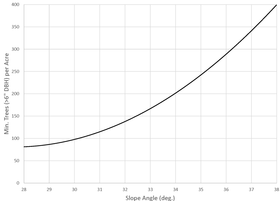
Figure 14 – Minimum Conifer Densities vs. Slope for Avalanche Protection
