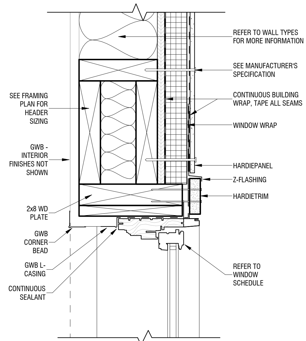
2 HARDIEPANEL TYP WINDOW HEADER 3" = 1'-0"
