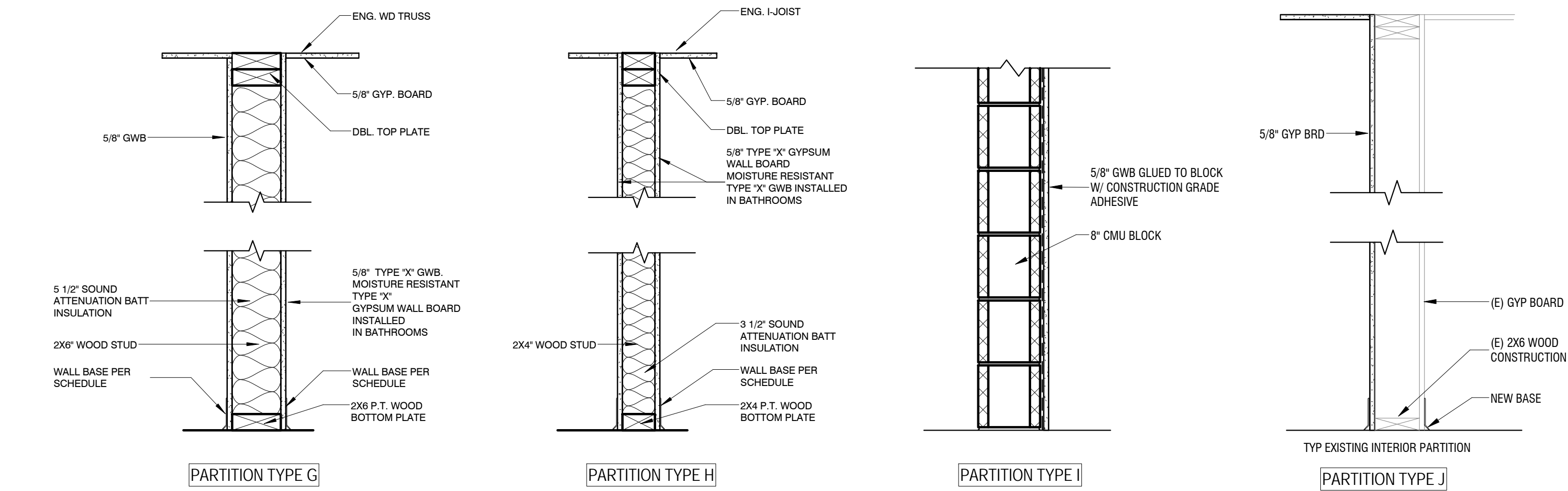
1 PARTITION TYPES 1" = 1'-0"
