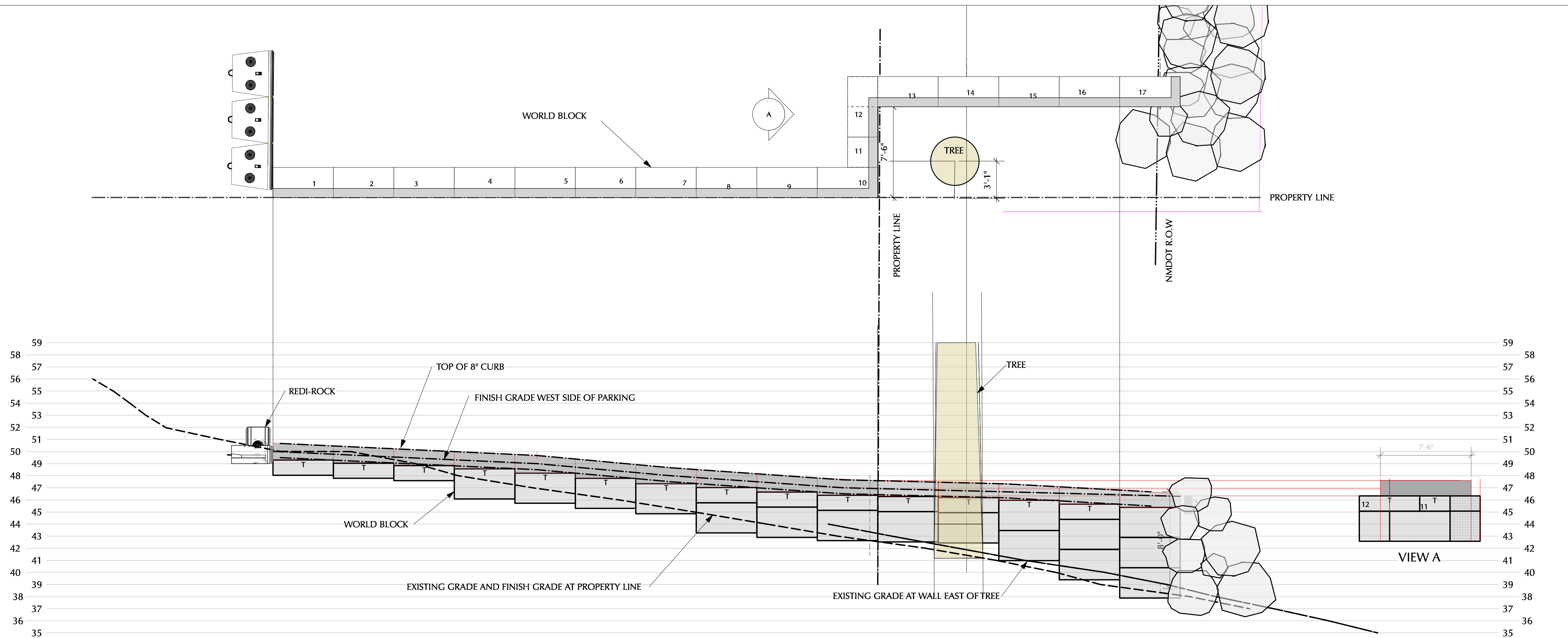
1 WEST RETAINING WALL PROFILE AND PLAN C-8 R2 Scale: 3/16" = 1'-0"
