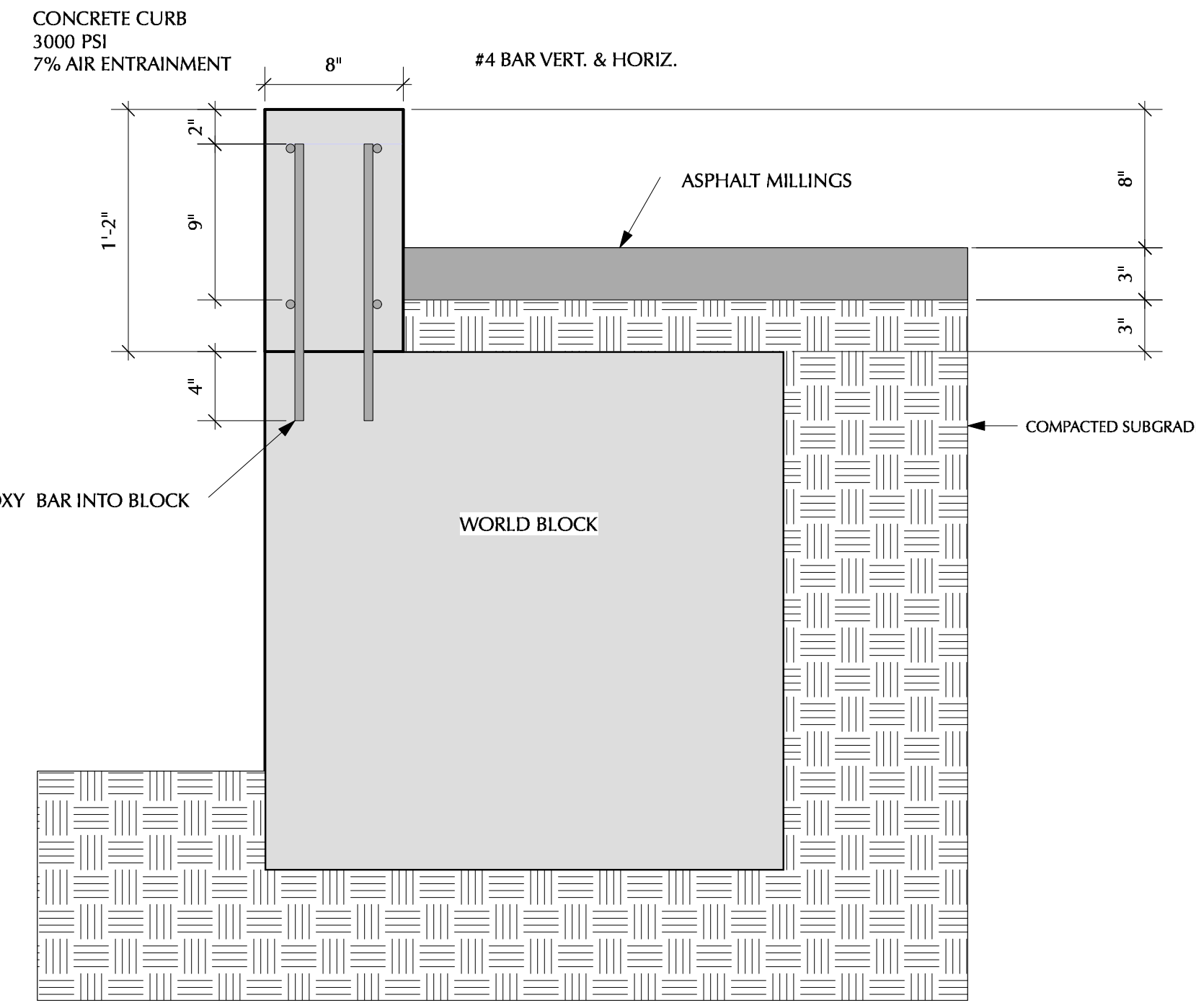
3 CURB DETAIL AT SOUTH END OF BLOCKS Scale: 1 1/2" = 1'-0"
