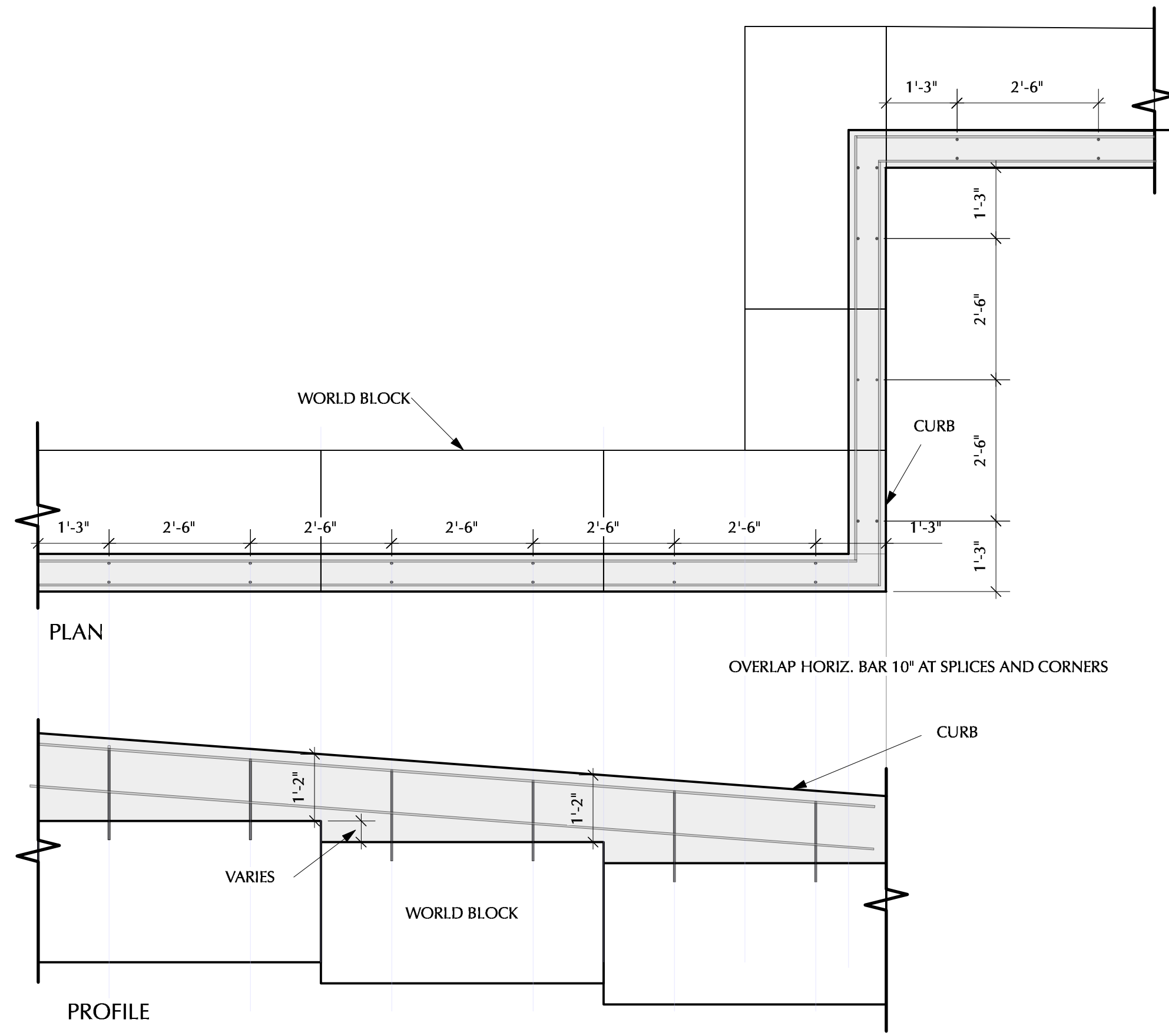
2 PLAN & PROFILE SW CORNER Scale: 1/2" = 1'-0"
