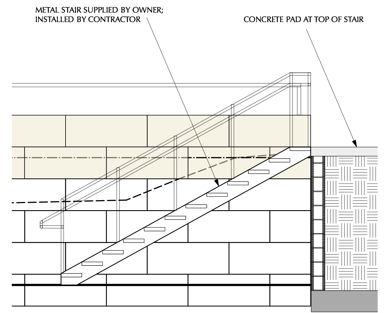
3 STAIR @ WEST WALL Scale: 3/8" = 1'-0"
