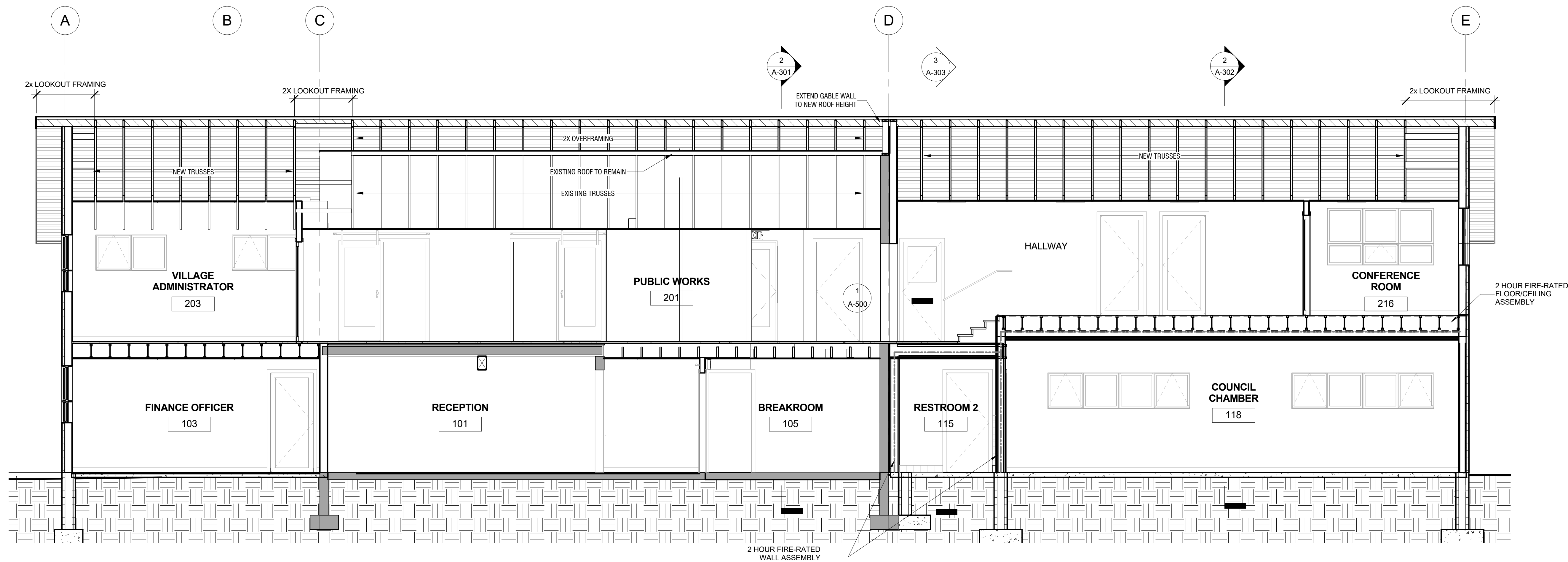
1 BUILDING SECTION 1 1/4" = 1'-0"
