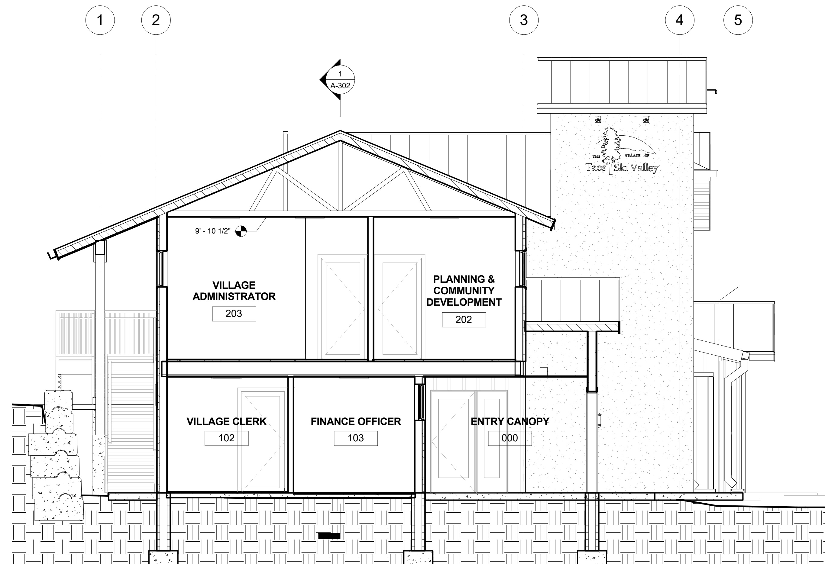
3 SECTION THROUGH ENTRY CANOPY 1/4" = 1'-0"
