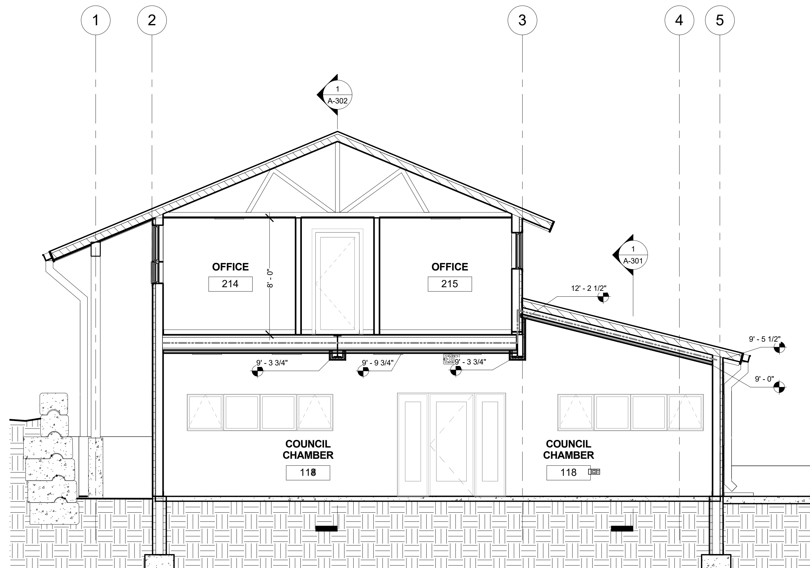
2 BUILDING SECTION 2 1/4" = 1'-0"
