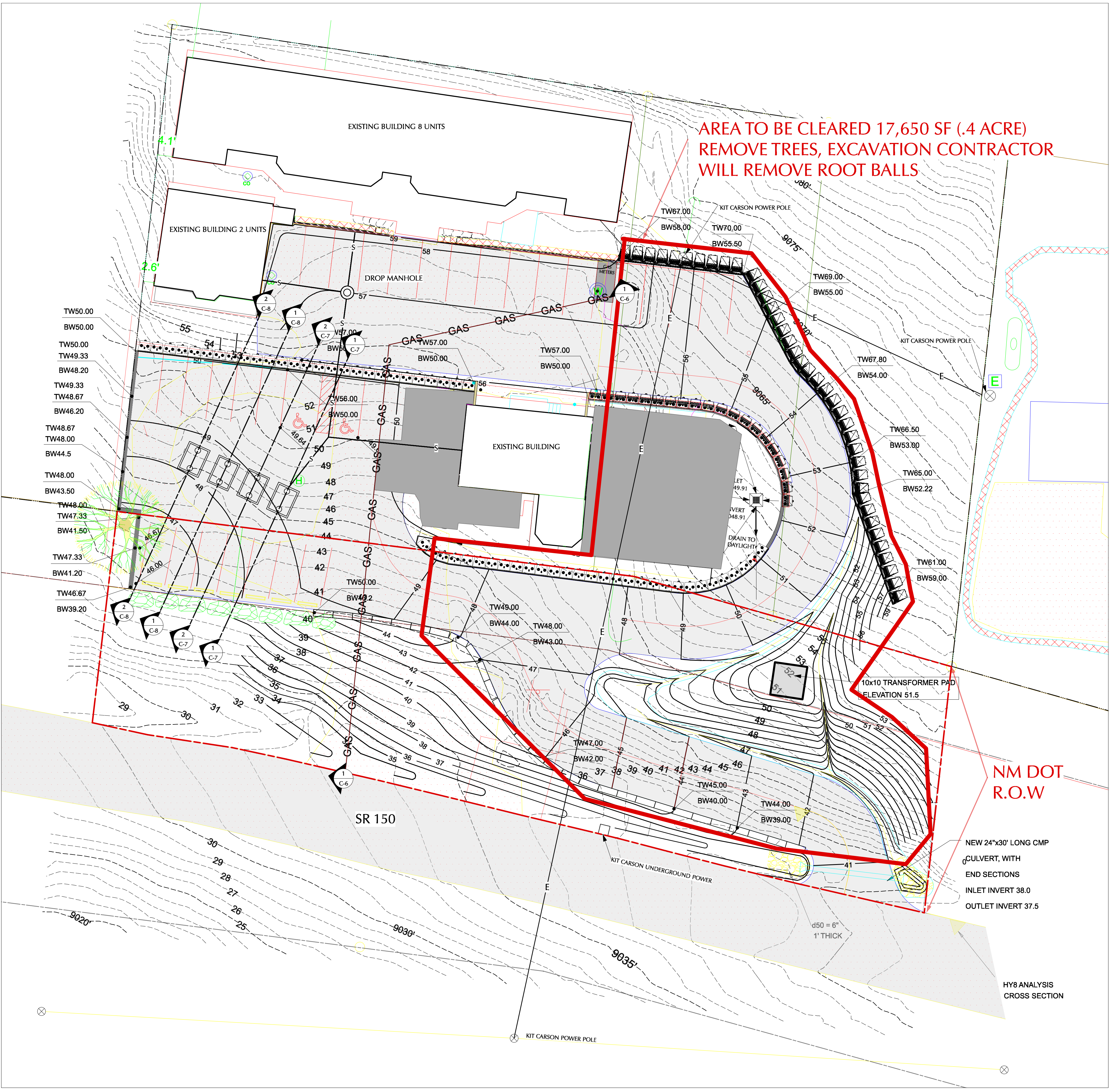
1 SITE CLEARING PLAN C-2.2 Scale: 1/16" = 1'-0"
