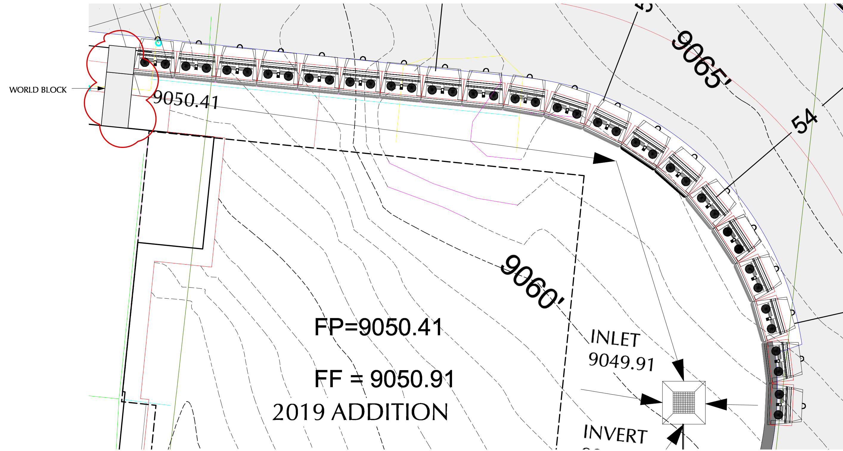
2 EAST UPPER WALL PLAN C-12 R Scale: 3/16" = 1'-0"
