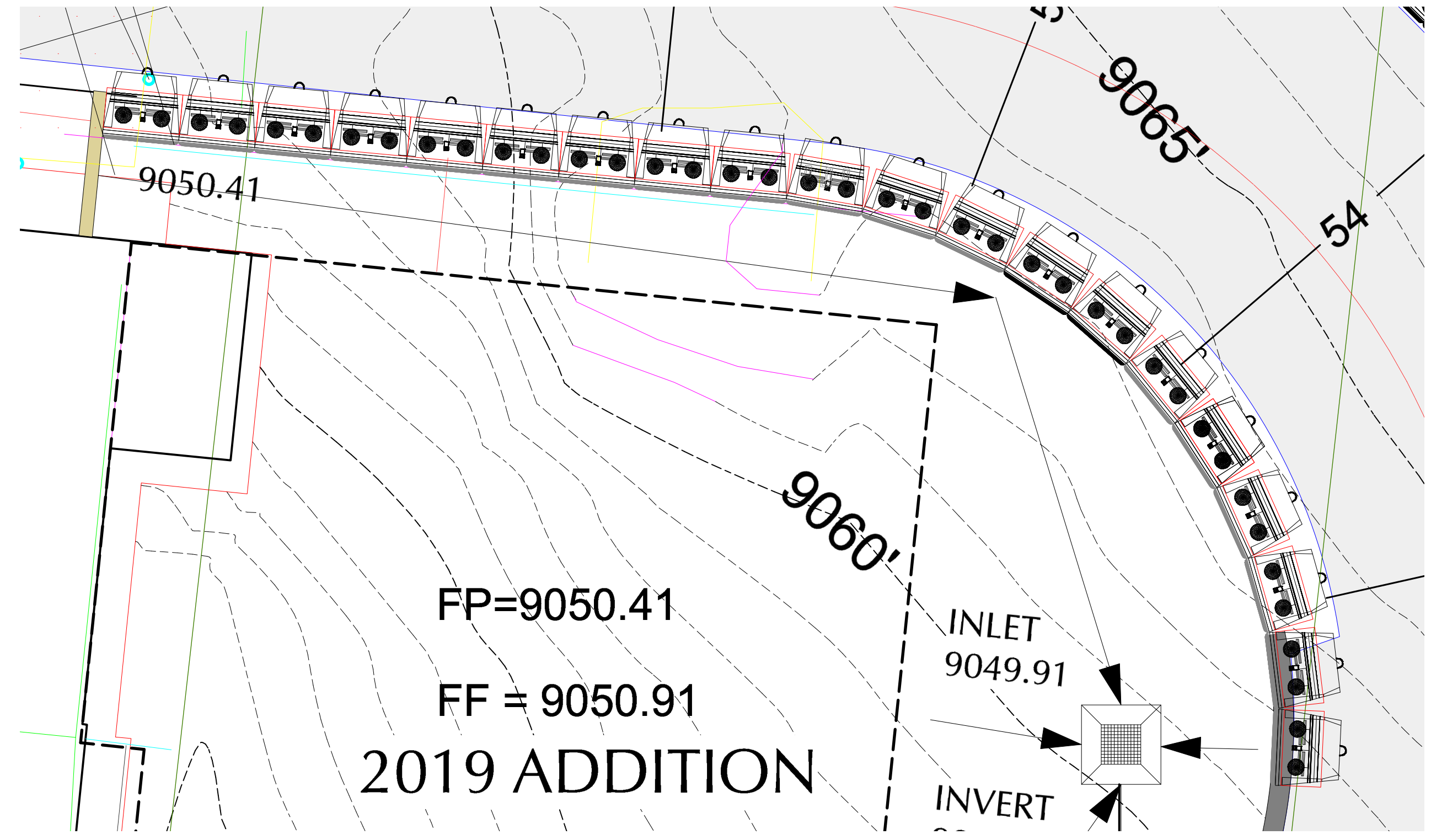
2 EAST UPPER WALL PLAN C-12 Scale: 3/16" = 1'-0"
